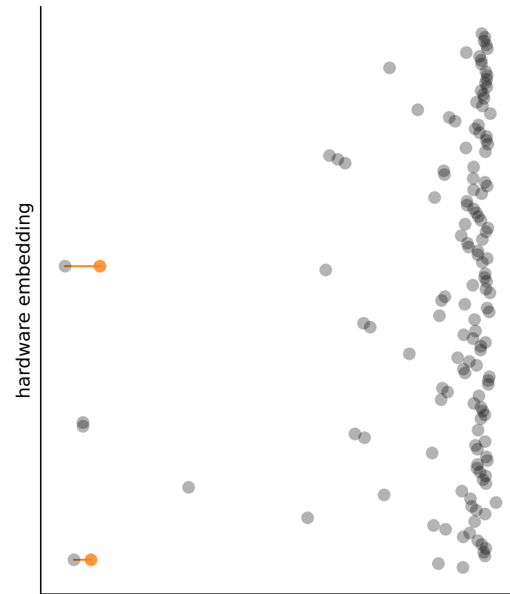
horizon = 5
