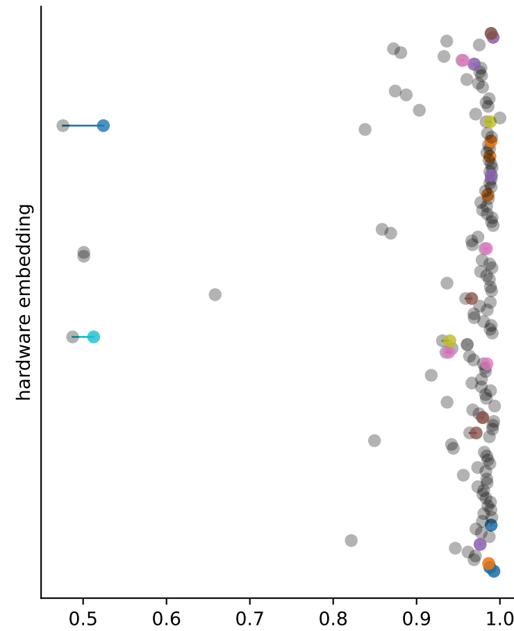
horizon = 8
